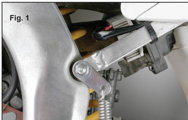
Honda 450X models reg/rec is located at the air-box
