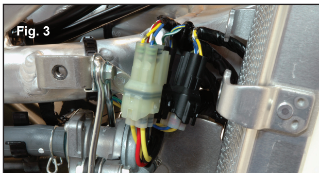
Steps 3) Trail Tech stator plugged in
