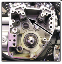
Verify Intake lobes of camshafts clear engine case Crank bearing boss & lifter bosses
