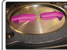
Measure valve to piston clearance clay pistons and measure thickness of clay after cycling engine
