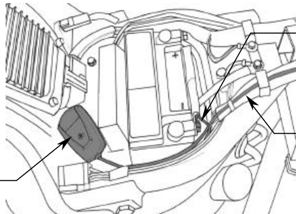
FIGURE 4 (07 SOFTAIL)
