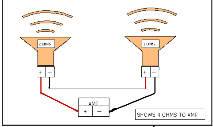
SERIES WIRING
