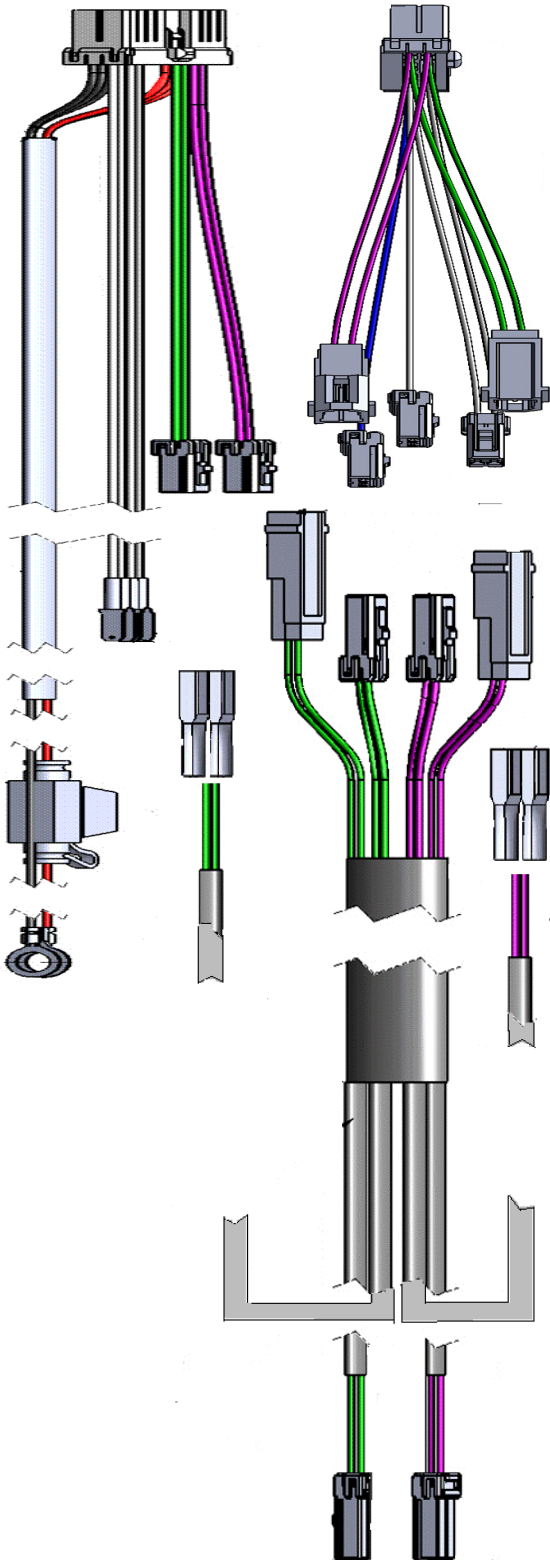
FIG 1 USE THESE HARNESSES AND Y CONNECTORS FOR TWO OEM/ KICKER FRONT SPEAKERS AND KURYAKYN SADDLEBAG LID SPEAKERS —MODIFIED EXTENSION HARNESS SHOWN
