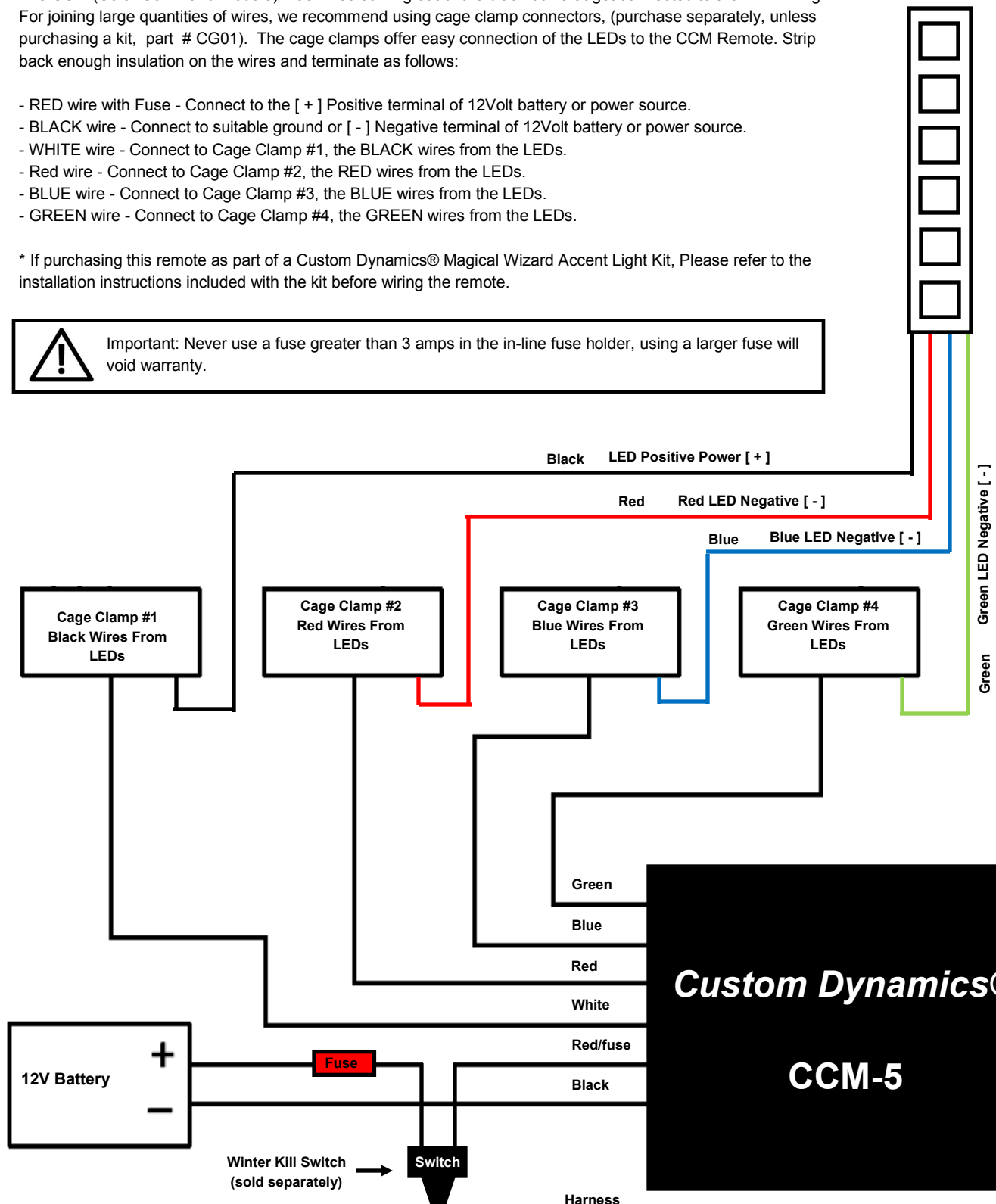
Magical Wizard™ 4 Wire LED Pod
